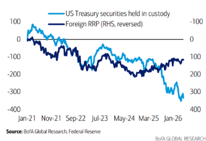
Exhibit 34: Cumulative change in custody holdings and foreign RRP UST securities held in custody are typically negatively correlated with foreign RRP take-up but we have seen some divergence since July '25
